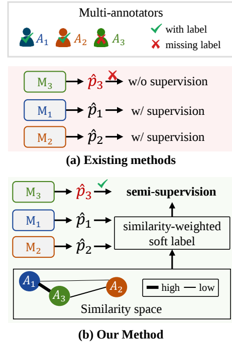
Figure 1: Comparisons. Three annotators label a video sample with different annotations, with the third annotator's label missing. (a) In existing methods, the predicted label distribution \hat{p}_3 from annotator 3's model M_3 lacks supervision due to the missing label, resulting in the model training being skipped without updates. (b) In contrast, our proposed method leverages similarities of annotators' labeling patterns derived from the dataset to generate a soft label \hat{p}_{3,soft} that closely approximates annotator 3's true label. This is achieved by applying similarity-weighted aggregation to the predictions \hat{p}_1 and \hat{p}_2 from other annotator models, enabling semi-supervised updating of models with missing labels.
