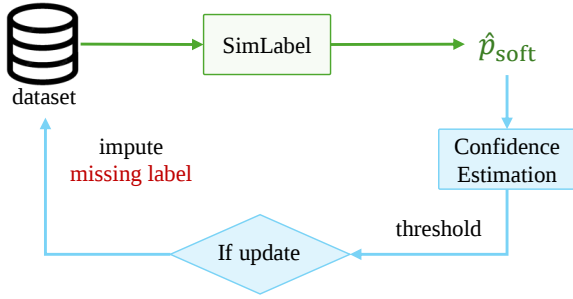
Figure 3: The confidence cycling of SimLabel. Confidence is calculated for the soft label ( \hat{p}_{soft} ) generated for missing labels. When confidence exceeds a predetermined threshold, the predicted label is obtained and used to impute the corresponding missing label in the dataset. The annotator similarity matrix derived from the dataset is iteratively updated and utilized for soft label ( \hat{p}_{soft} ) generation in subsequent iterations.
